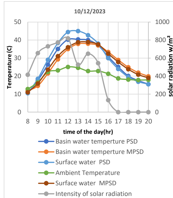
Figure ( 9 ) shows the temperature difference between the water surface and the base of the two regular and improved pyramid devices with the intensity of solar radiation and the ocean temperature for to day 12/10/2023.
