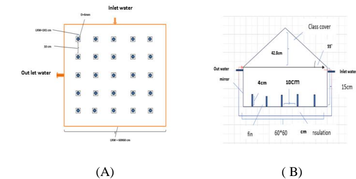
Figure (4) : (A) shows the detailed diagram of the base of the improved solar still, (B) shows plan of what the device looks like from the outside.
