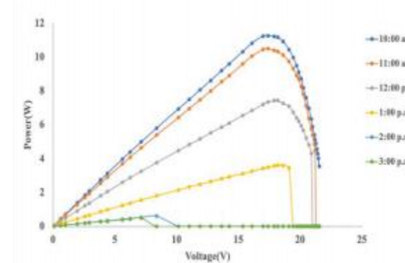
Figure 14: Power-Voltage Curve (MPPs9) for Both SASTS & Simulation
