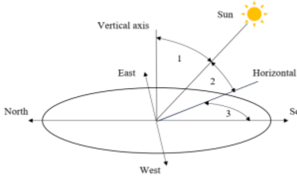
Figure 3: Sun Radiation Angles Simulation 1: Zenith angle 2: Altitude Angle ( \alpha = 35^\circ ) 3: Azimuth Angle
