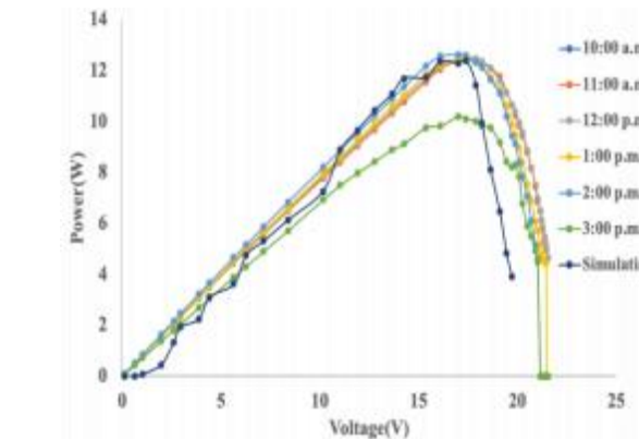
Figure 13: Current-Voltage Curve for Both SASTS & Simulation
