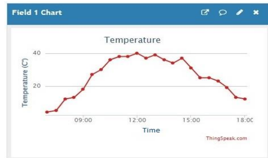
Figure 7. The displayed temperature on ThingSpeak
