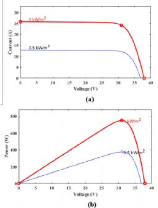
Figure 4. PV array characteristics affected by irradiance at 25°C (a) I-V, (b) P-V
