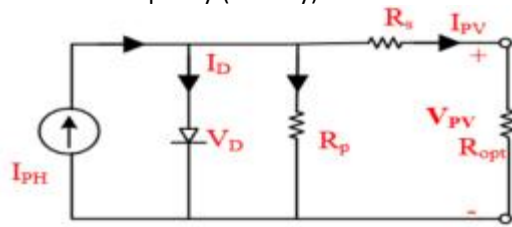
Figure 3. Single-diode circuit model of PV cell
