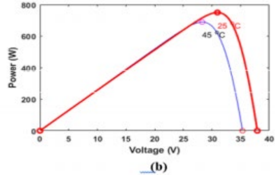
Figure 5. PV array characteristics affected by temperature at 1000 Kw/m² (a) I-V, (b) P-V
