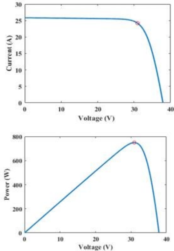
Figure 7. I-V and P-V characteristics of typical photovoltaic under STC (25°C and 1000 W/m 2 )
