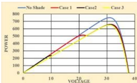
(a) P-V Curves
