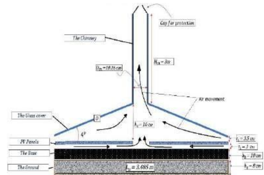
Fig. 5 Dimensions of the experimental model
