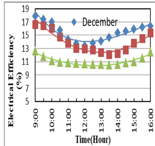
Fig. 16 The change of the hourly electrical efficiency during the day.
