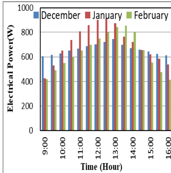
Fig. 14 Variation of the electric power during the day for different months
