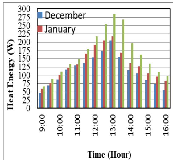
Fig.15 Variation of the heat power during the day for different months
