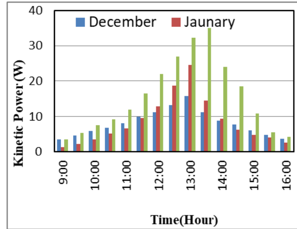
Fig. (13) Kinetic Power Variation.
