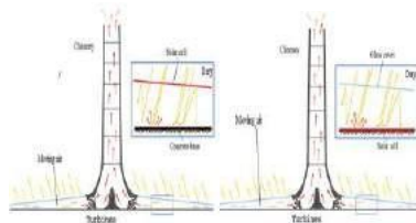
(a) The first model (b) Second design
