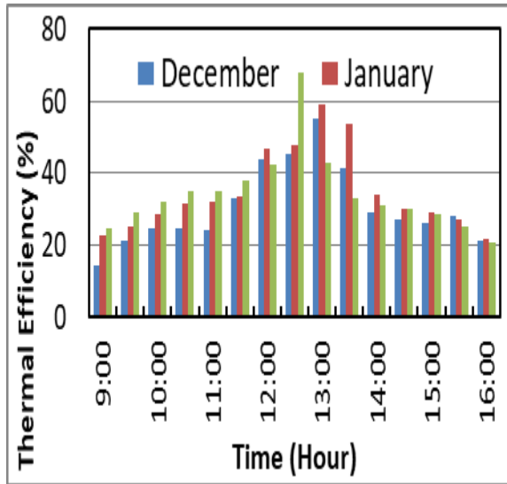
Fig. 17 The change of the hourly thermal efficiency during the day
