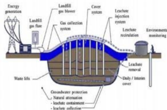
Fig (4) A typical engineered landfill with biogas recovery system [48].
