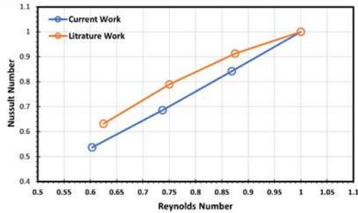
Figure(6) variation of Nusselt number with Reynolds number for smooth tube.
