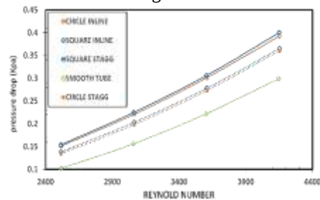
Figure(12) variation of pressure drop with Reynolds number for different pits shapes and arrans
