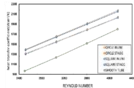
Figure(11) variation of heat transfer coefficient with Reynolds number for different pits shapes and arrangements.
