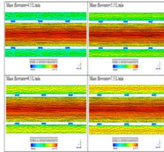
Figure(9) Velocity vector and contour of the fluid in shell and tube heat exchanger with pit on the internal surface of the shell
