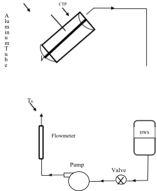
Fig (1): Solar collector with its main contents
