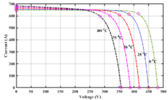
Fig(8) I-V Characteristic of the array at 1000 w/m2
