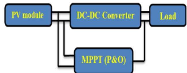
Fig (1) Overall block diagram
