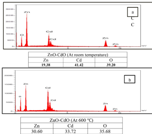
Figure 3: EDXA of ZnO:CdO (a) at Room Temperature, (b) at 600 °C
