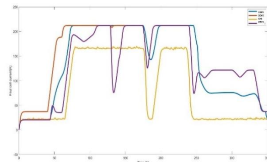
Figure 4: Fuel Cell Current Over Time
