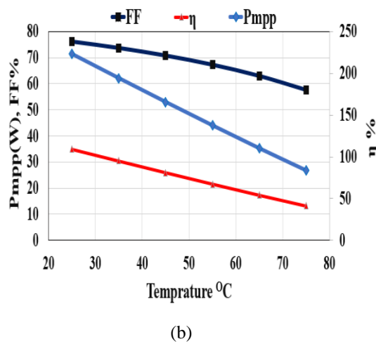
Figure 5. Effect of temperature change on (a) VO.C, Vmpp, Is.c, Imp (b) Pmpp, FF, \eta [28]
