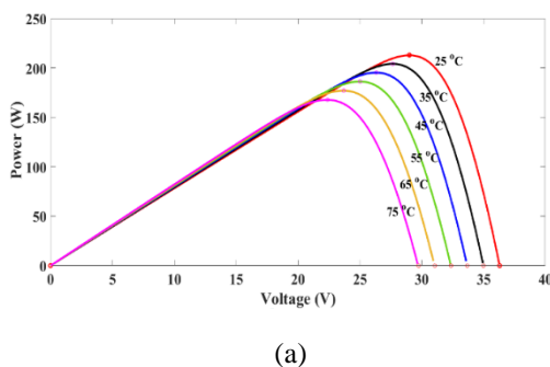
Figure 5. Effect of temperature change on (a) VO.C, Vmpp, Is.c, Imp (b) Pmpp, FF, \eta [28]
