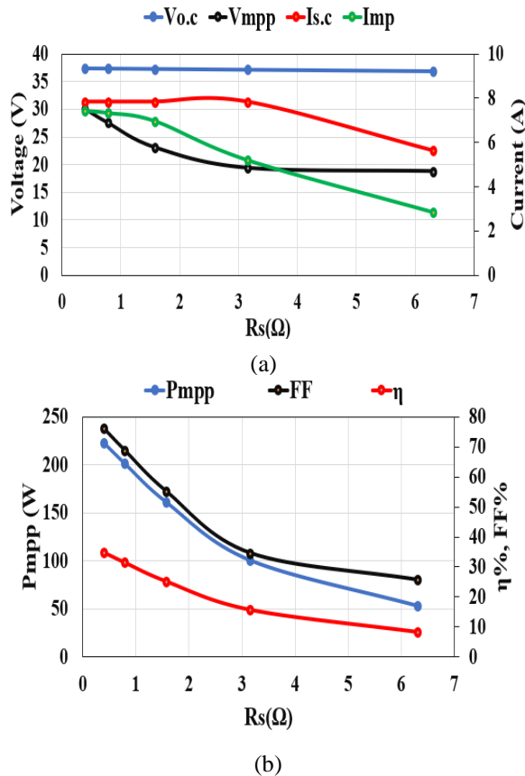
Figure 9. Effect of R_s change on (a) V_{OC} , V_{mpp} , I_{sc} , I_{mp} (b) P_{mpp} , FF, \eta [14]
