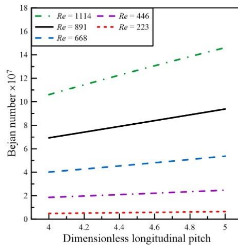
Figure 10. Influence of Bejan number on the dimensionless longitudinal pitch for various Reynolds numbers.
