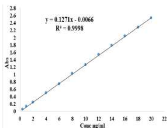
Figure. 3: Standard curve for the determination of HCTZ using nitrogenase and conjugation.
