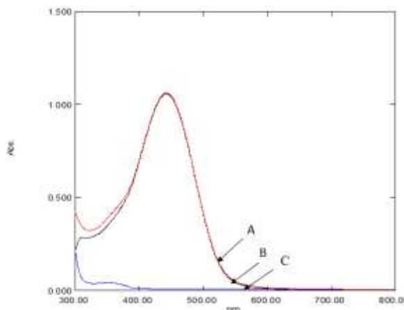
Figure. 2: Final absorption spectrum of 8 µg/25 mL of a nitrogenized HCTZ solution. (A): vs. mock solution, (B): vs. distilled water, (C): mock solution versus distilled water.
