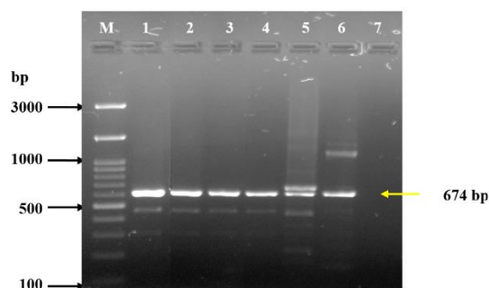
Figure 5. Agarose gel electrophoresis to detect the coa gene of MRSA with a size of 674 bp. Lane M represents the DNA ladder, lanes 1-6 represent positive samples, lane 7 represents the negative control.
